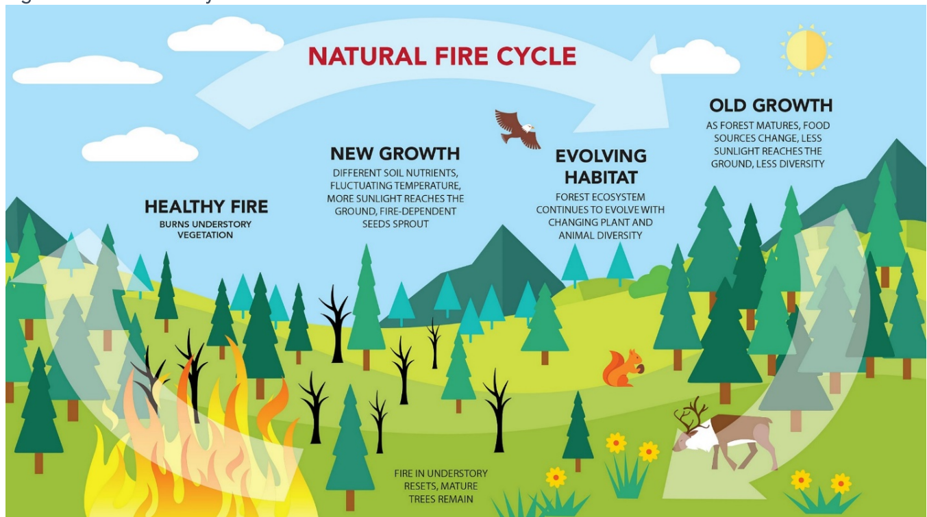
Figure 2. Natural Fire Cycle
