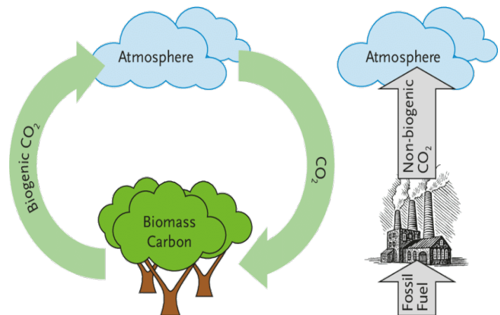
Figure 1. Terrestrial Carbon Cycle vs Fossil-Fuel Combustion
